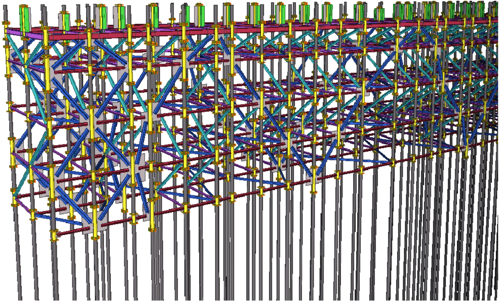
World Trade Center Transportation Hub Minipiles and Bracing New York, NY
