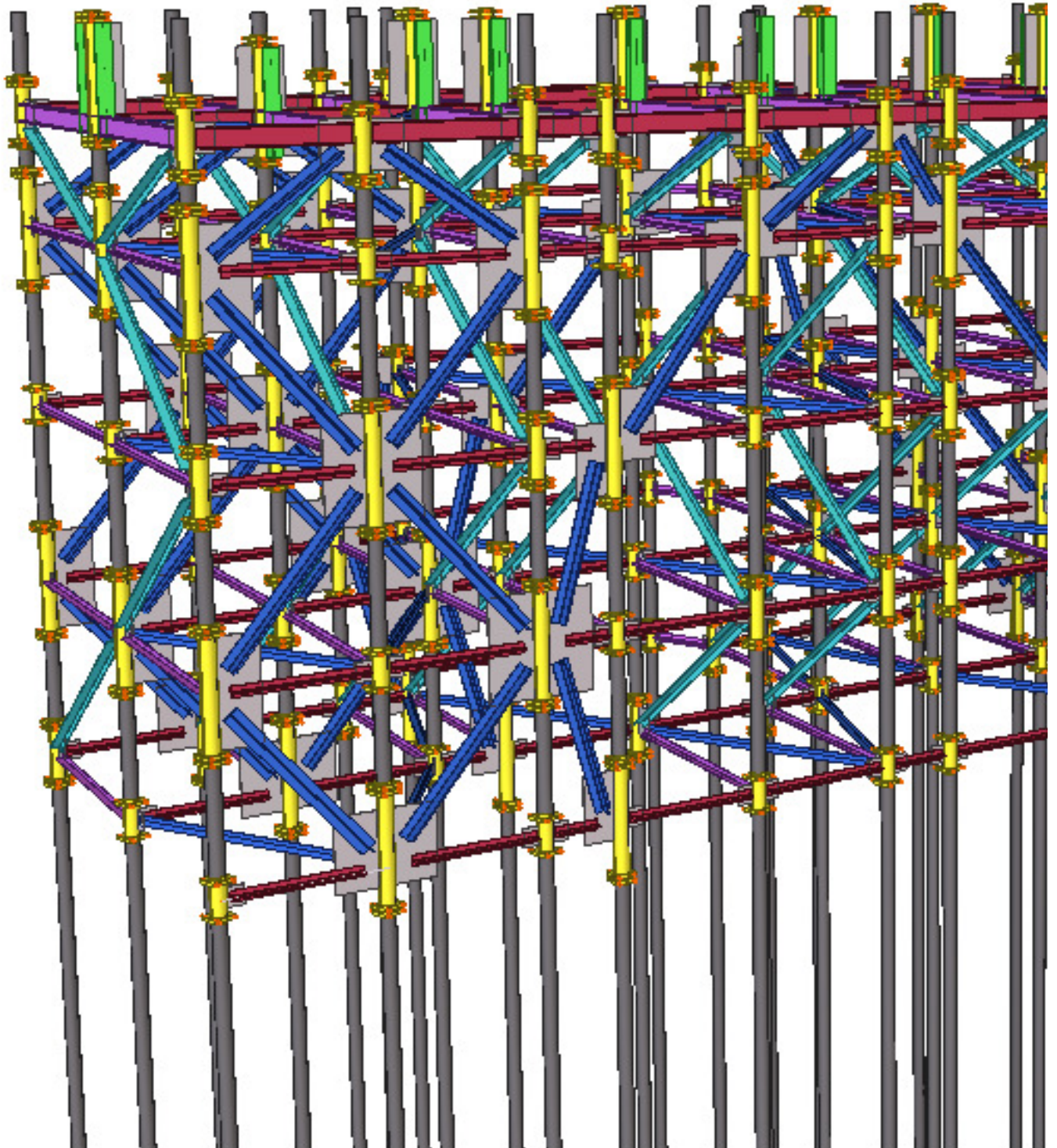
World Trade Center Transportation Hub Minipiles and Bracing New York, NY
