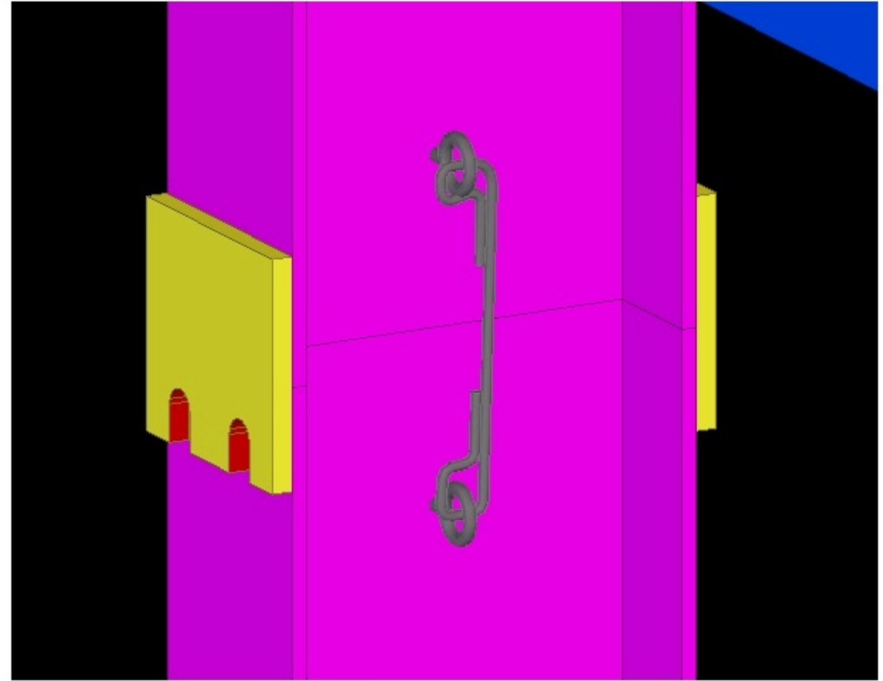
DETAIL - A
