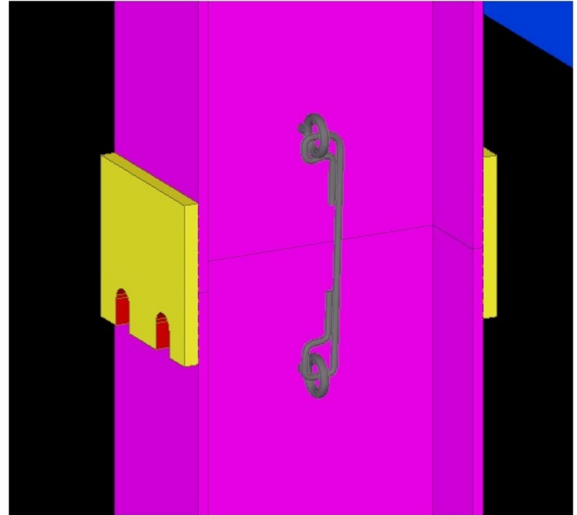
DETAIL - A
