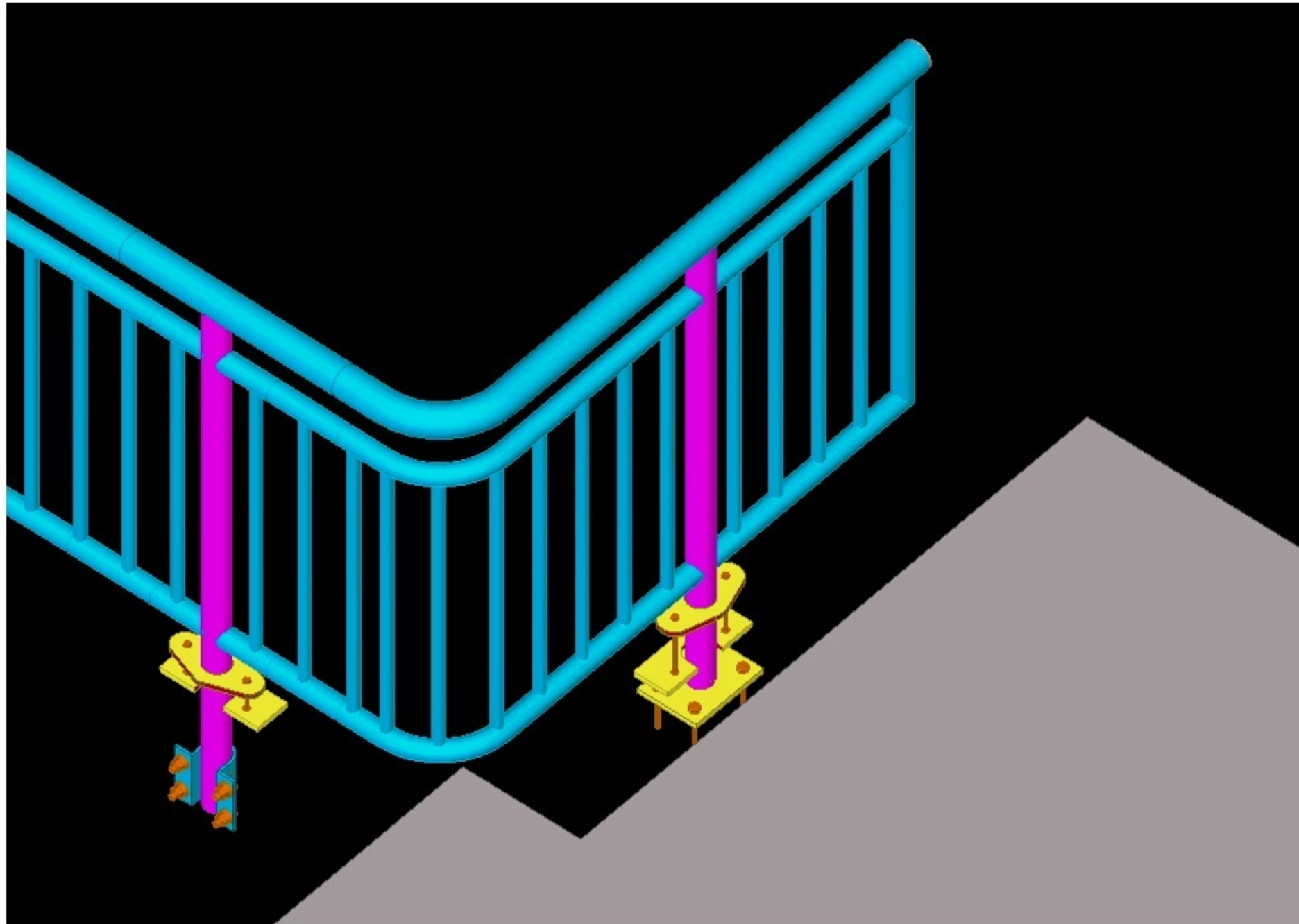
DETAIL - A
