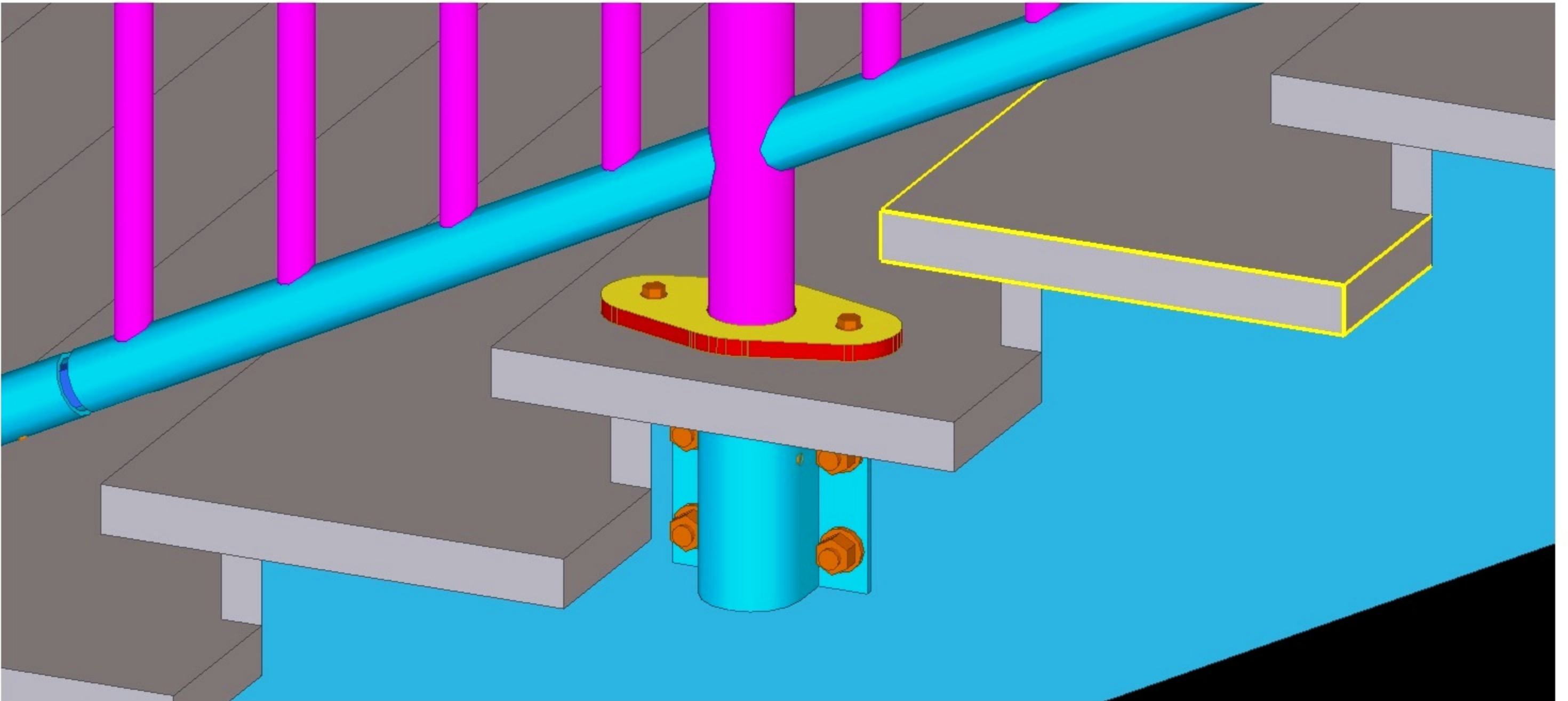
DETAIL - A
